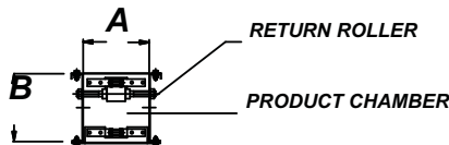
CROSS SECTION TYPICAL TROUGH
